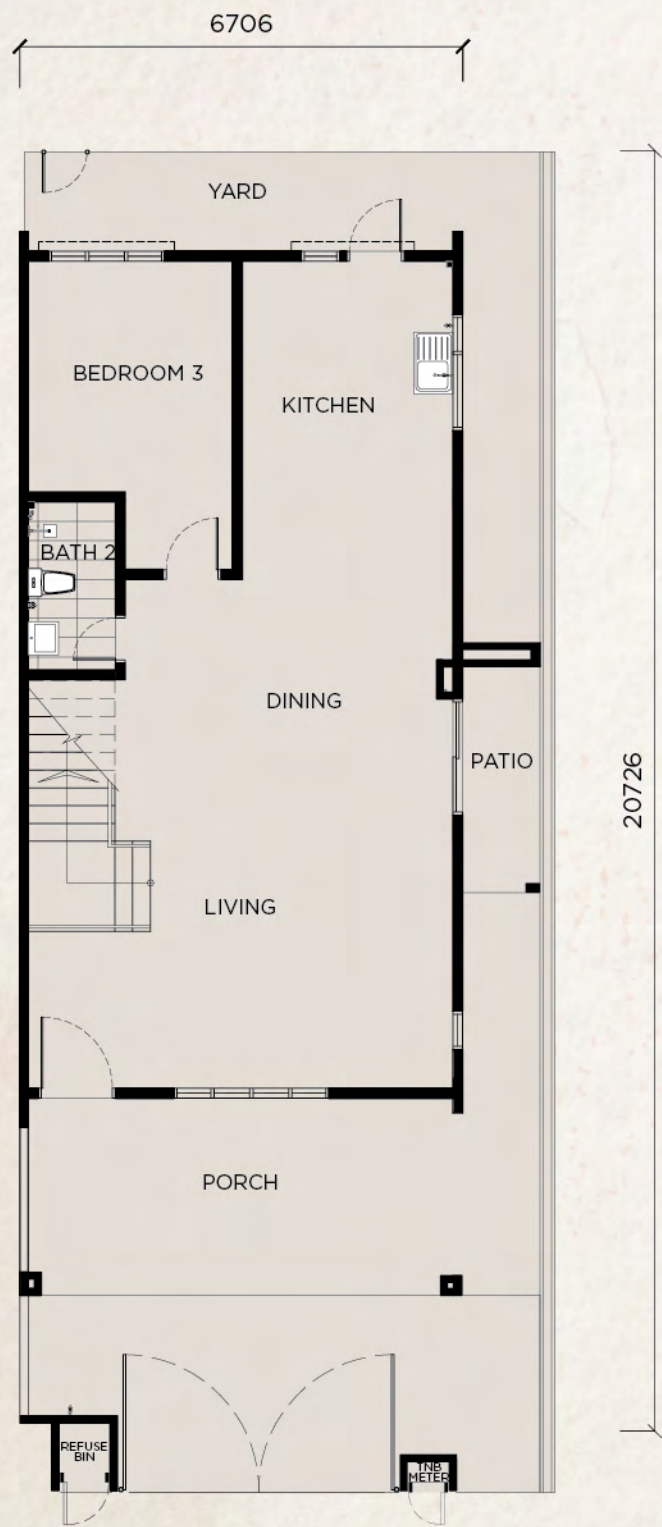
GROUND FLOOR
